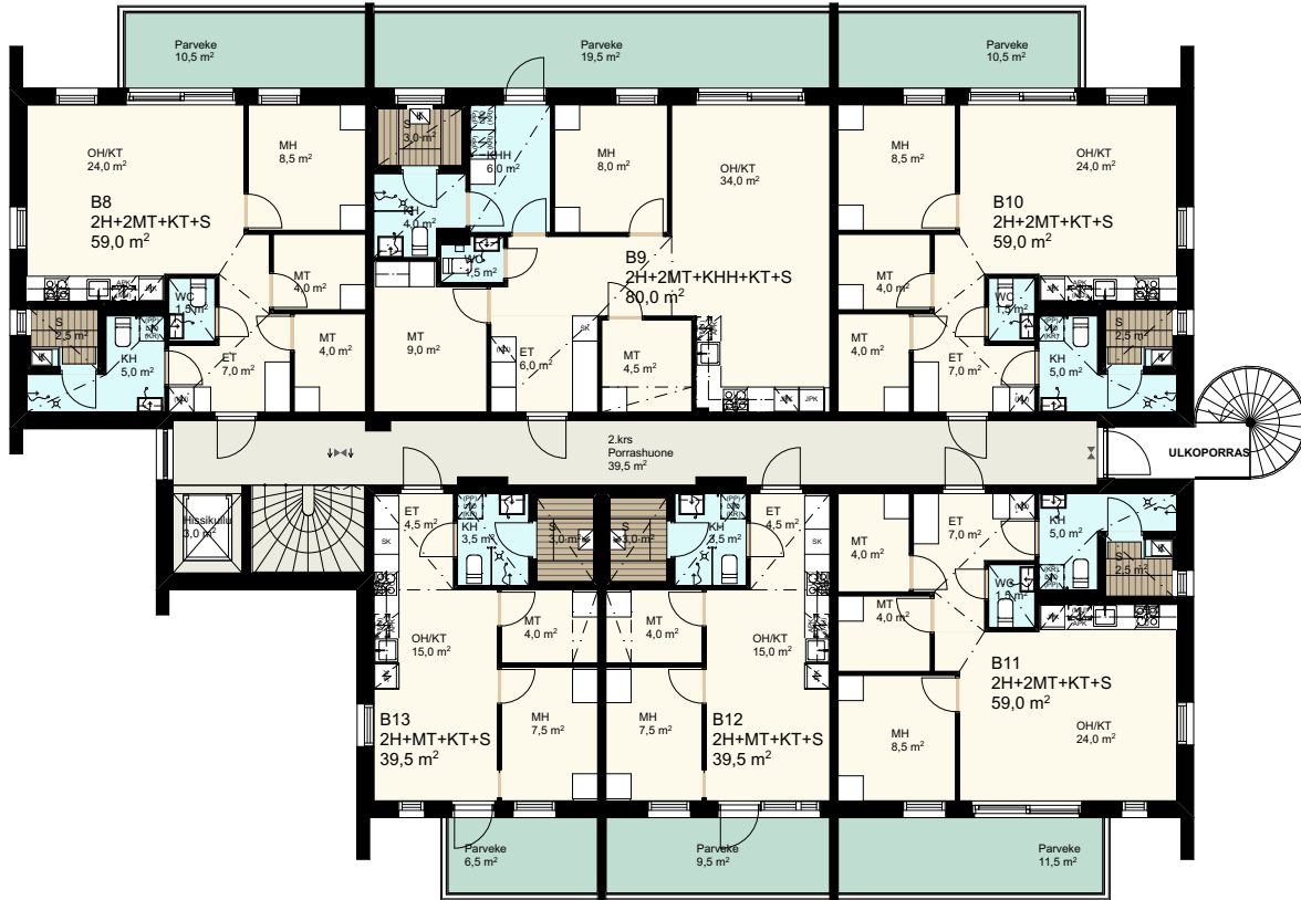
Talo B - 2. krs
