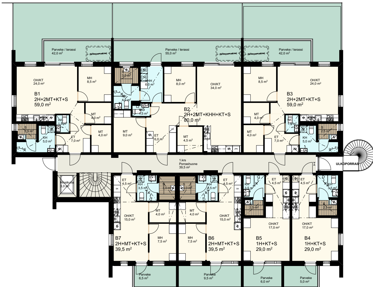
Talo B - 1. krs
